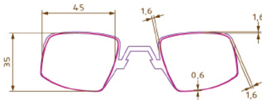
Optical insert Ref. IRISRXXKIT
